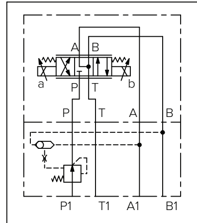
BYPASS - 3 WAY
