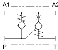
Schematic Symbol
