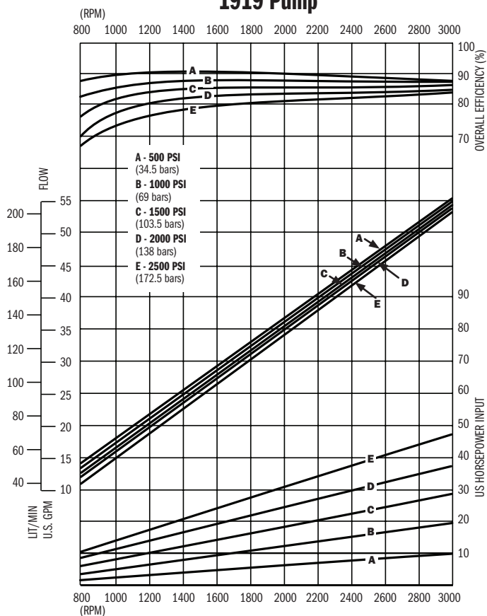
1919 Pump
