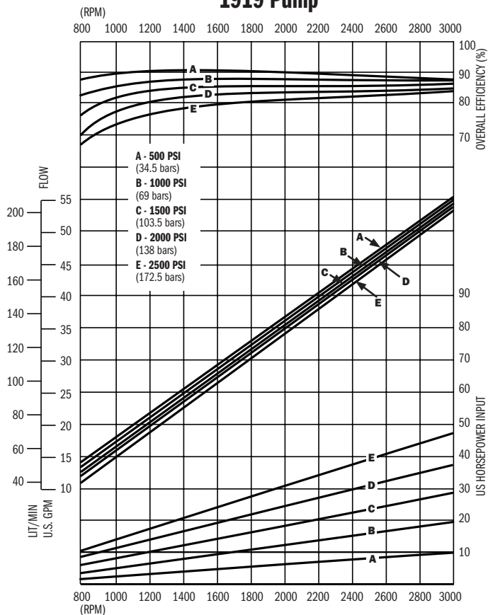
1919 Pump
