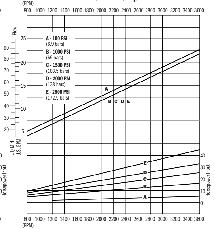
1512K Pump
