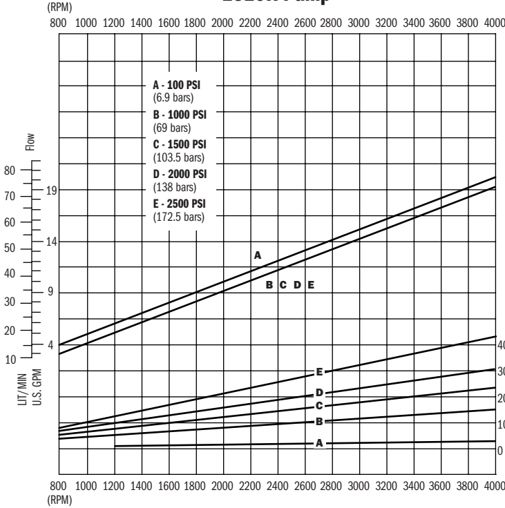
1510K Pump
