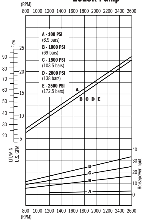
1518K Pump
